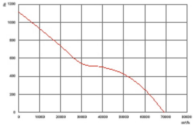
NFDAX/BX 1000-8-45
