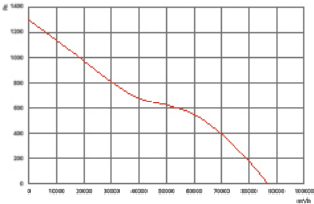
NFDAX/BX 1120-8-40
