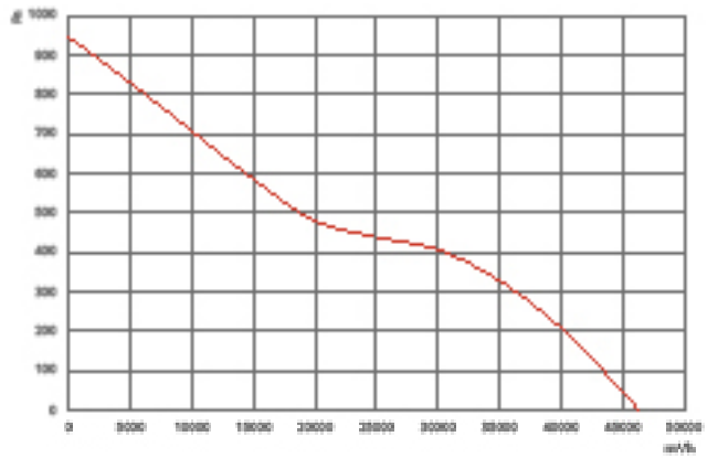
NFDAX/BX 900-8-40
