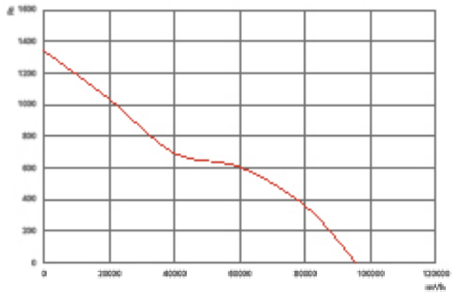
NFDAX/BX 1120-8-45
