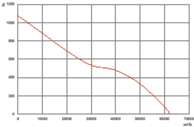
NFDAX/BX 1000-8-40
